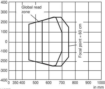
Reading characteristics VB34*OM*
